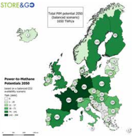
POWER-TO-METHANE POTENTIAL 2050 – STORE&GO
