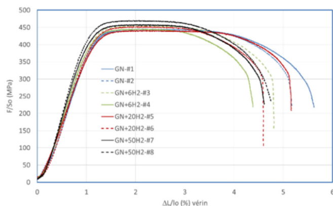
Tensile curves results for pure copper alloy on smooth specimens (Briottet and Portra, 2017).
